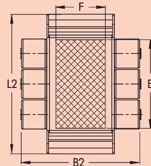
Sketch JFB 120 H
