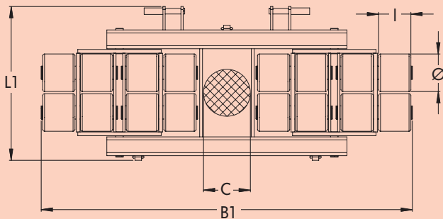
Sketch JFB 80 H
